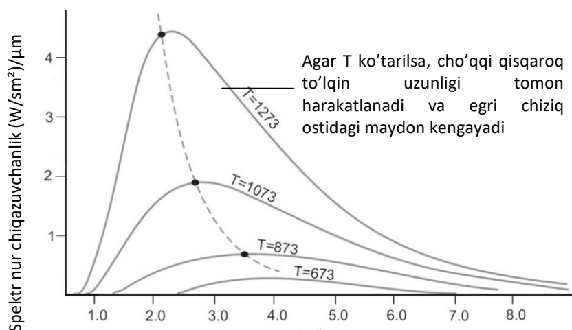
2.4-rasm. Stefan – Boltsman qonuniga asoslangan absolyut qora jism nurlanish egri chizig‘i (K haroratda), (Manba: 6 adabiyot).
