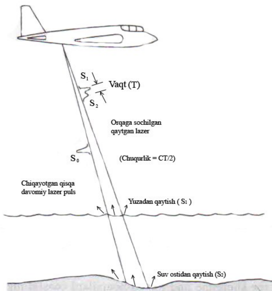
4.8-rasm. Lidar batimetriya (chuqurlikni o'lchash) tamoyillari (Manba: 6 adabiyot)
