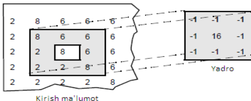
6.16-rasm. Namunaviy ma'lumotga 3 \times 3 o'rama yadro qo'llangan (Manba: 5 adabiyot).
