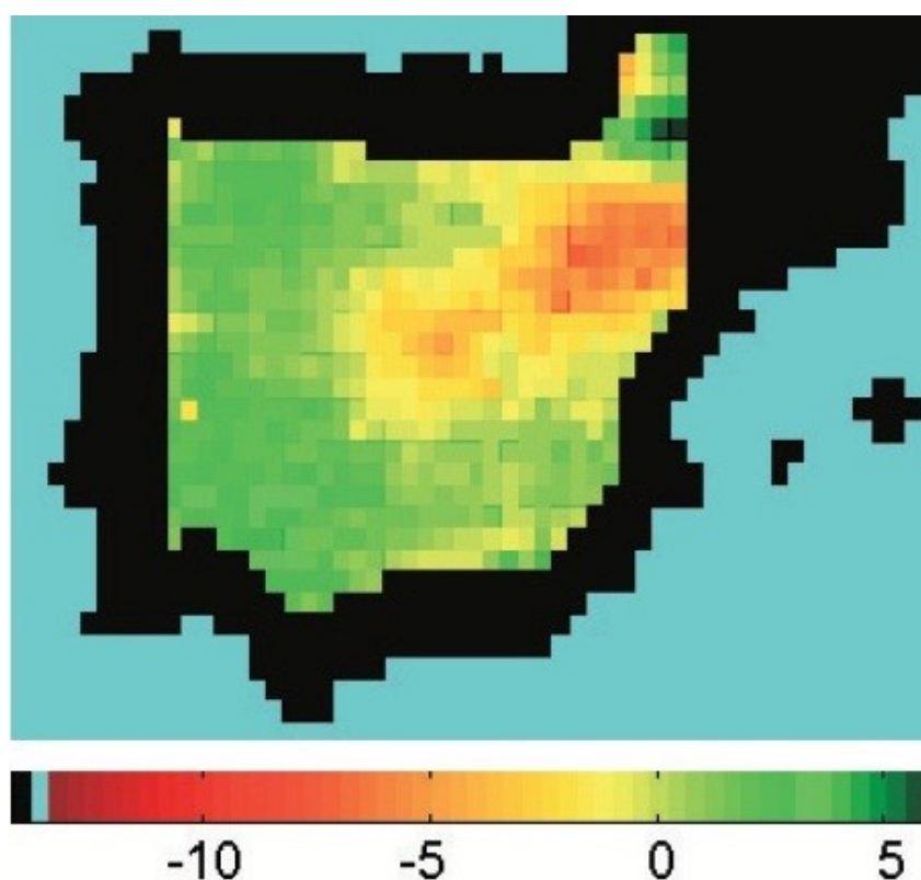
3.7-rasm. Iberiy yarim orolining 10 yil mobaynida tuproq namligining o‘zgarish kartasi(Manba: 6 adabiyot).
