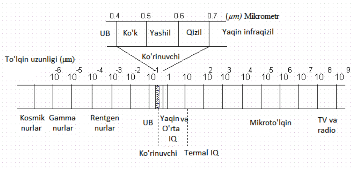
2.5-rasm. Elektromagnit spektr (Manba: 6 adabiyot).
