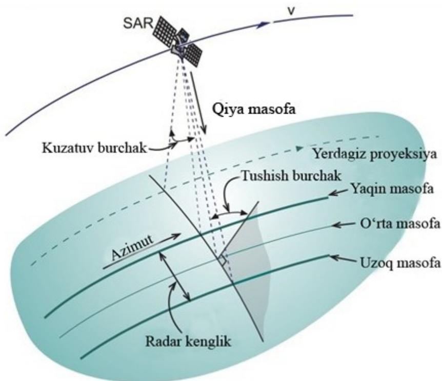
4.4-rasm. Radar masofadan zondlash geometriyasi(Manba: 6 adabiyot).
