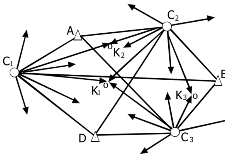
2.8-rasm. Ozod bekatlar taxeometriyasini bajarish sxemasi
