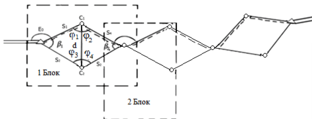
2.10-rasm. Taxeometrik yo'lining sxemasi
