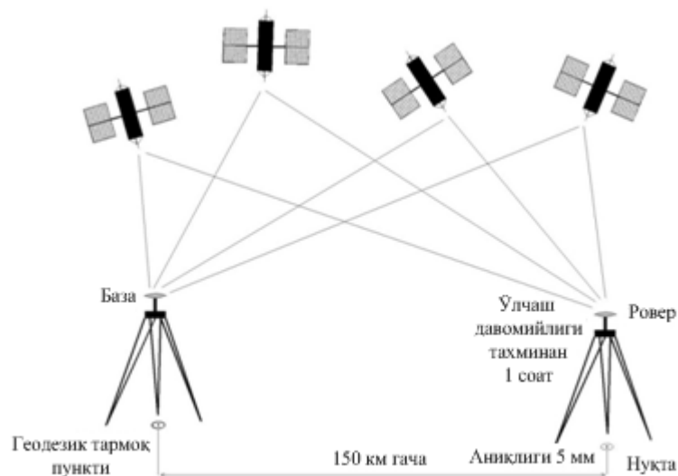
3.8-rasm. Statika usuli
