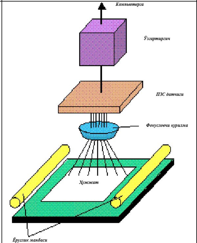
5.2-rasm. Proektsion skaner va uning ishlash sxemasi
