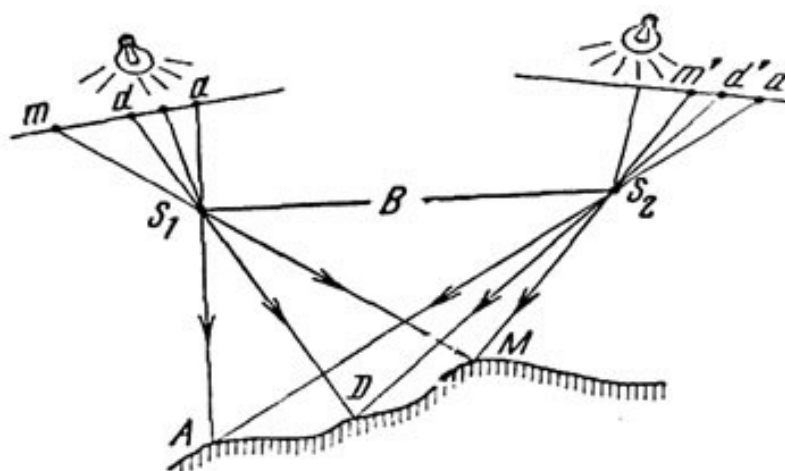
4.24-rasm. Joyning geometrik modeli
