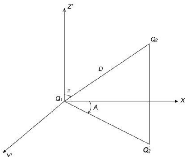
1.6-rasm. Topotsentrik gorizontalar sistemasida
